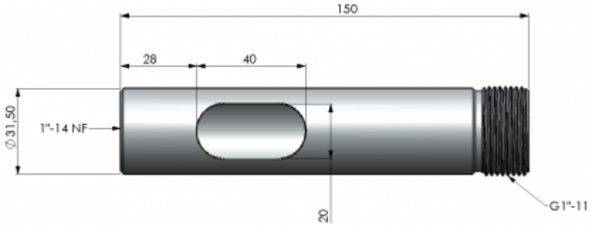
Outline Drawing
